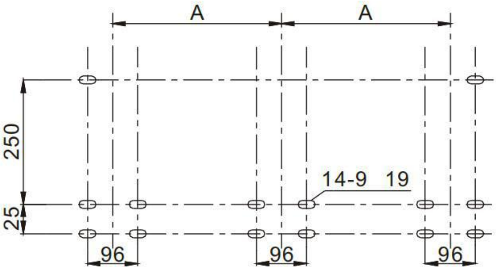
Mounting hole
