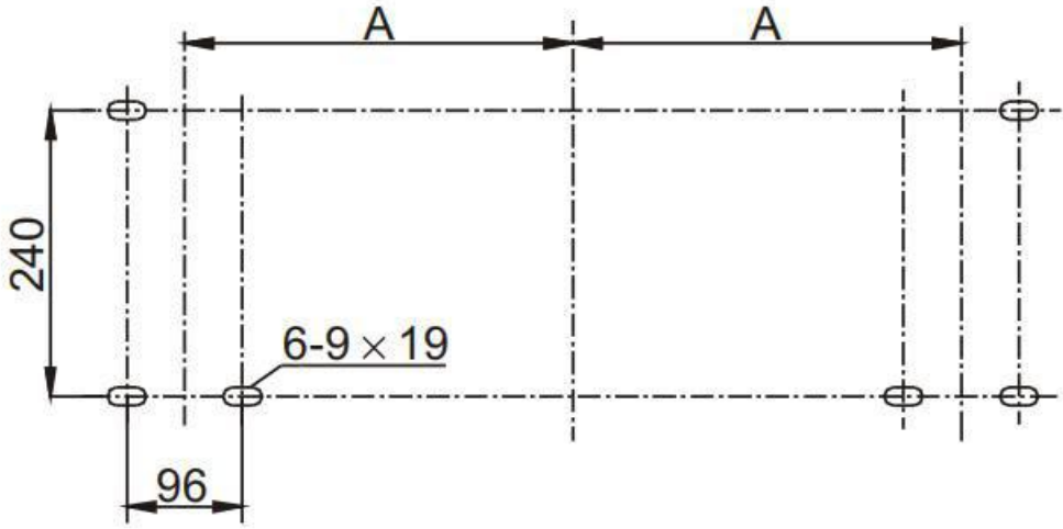
Mounting hole
