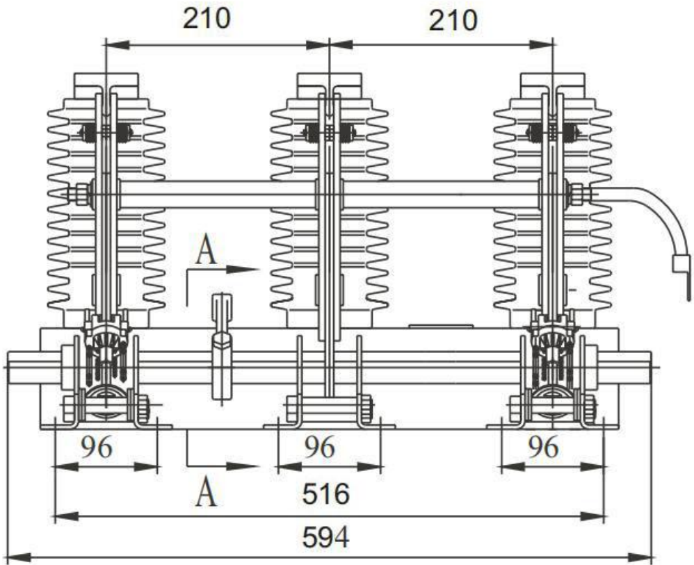
JN15-24/40 Earthing switch
