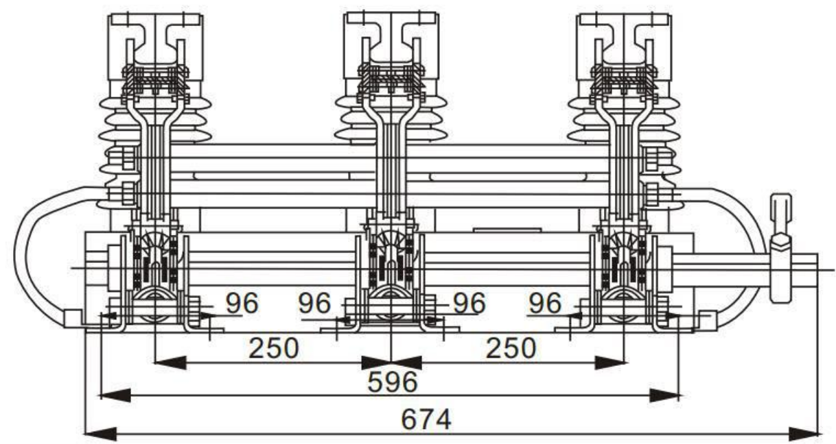
JN15-12/31.5 Earthing switch
